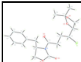
Fig. 1. The molecular structure of the title compound, showing the labelling of all non-H atoms. Displacement ellipsoids are shown at the 30% probability level.
